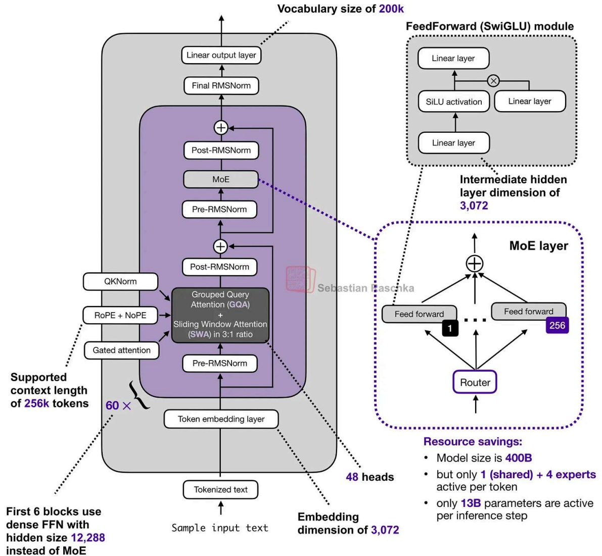
Figure 1: Overview of the Trinity Large architecture (based on the model hub config file ).
