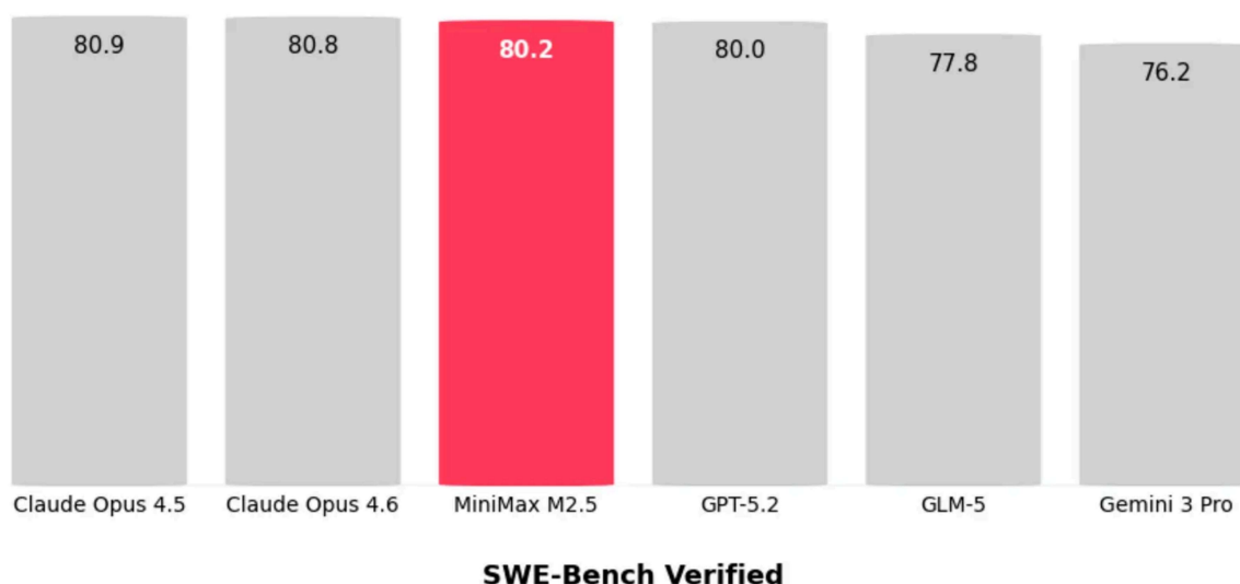
Figure 24: MiniMax M2.5 coding performance on SWE-Bench Verified
